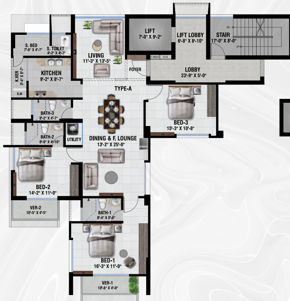
TYPE-A 5TH FLOOR PLAN 2141 SQFT N
